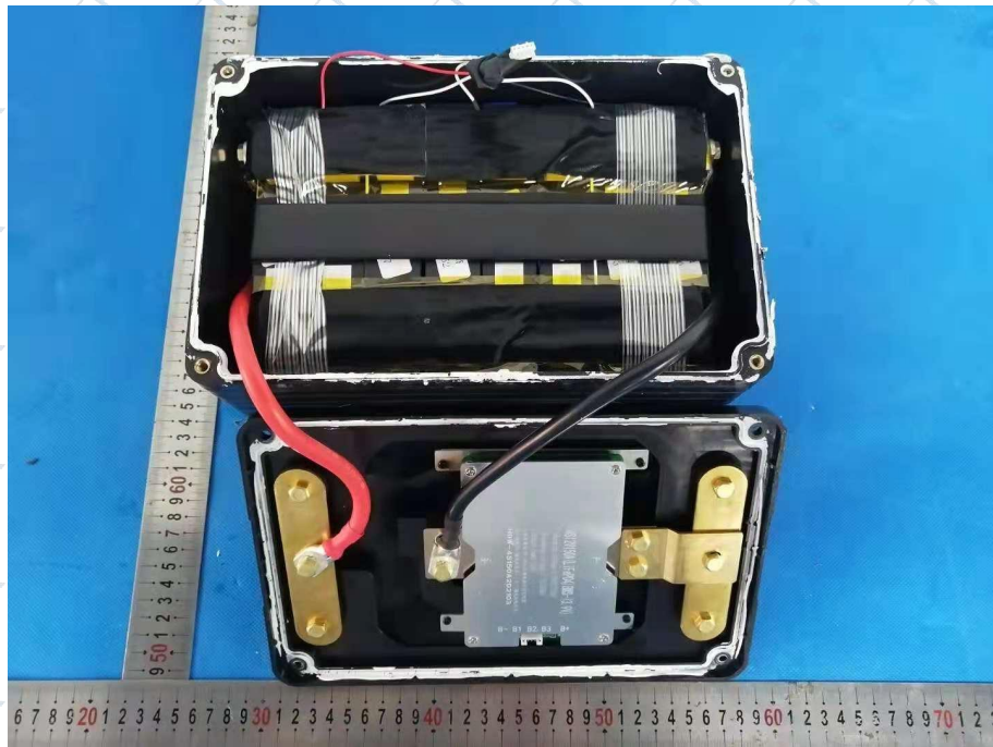
Photo 5 -- After test
